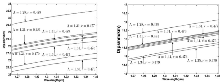
Figure 3 Dispersion Parameter D Variation Corresponding With the Wavelength at O Band
