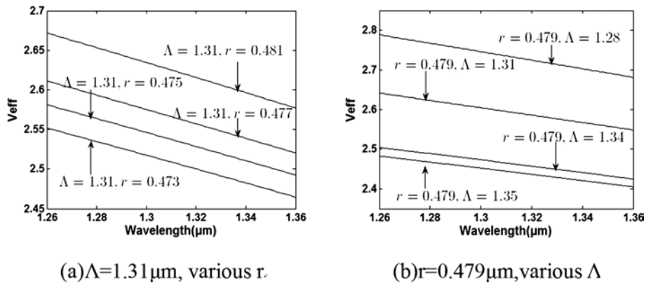
Figure 2 Effective Refraction V_{eff} Variation Corresponding with Wavelength
